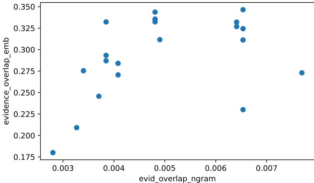
evid_overlap_ngram vs evidence_overlap_emb Spearman rho=+0.410 (moderate), n=20
