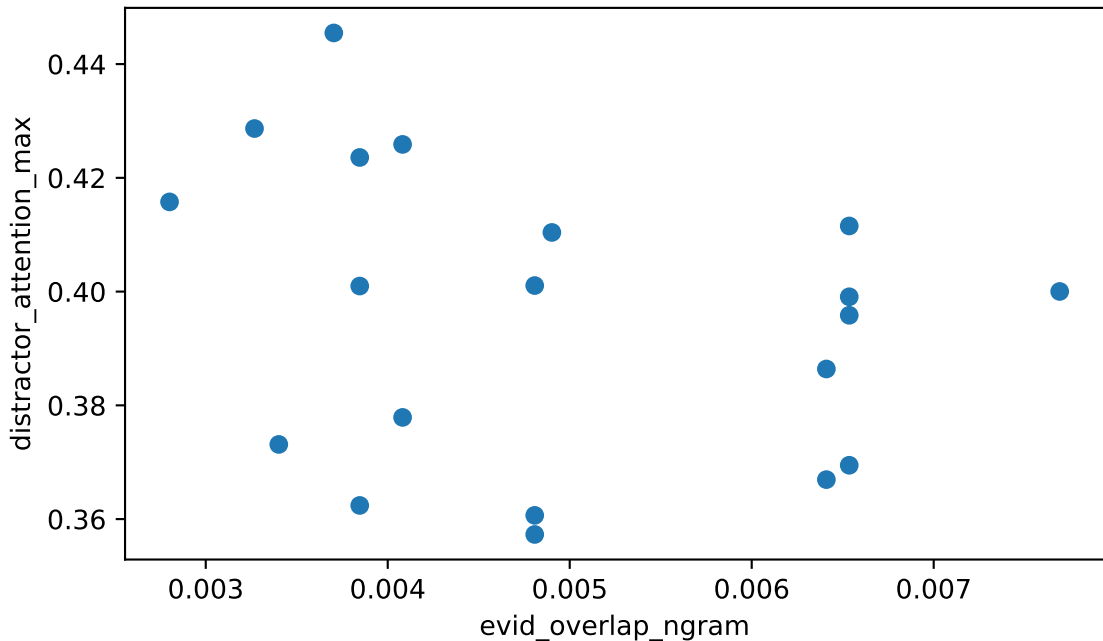
evid_overlap_ngram vs distractor_attention_max Spearman rho=-0.324 (weak), n=20
