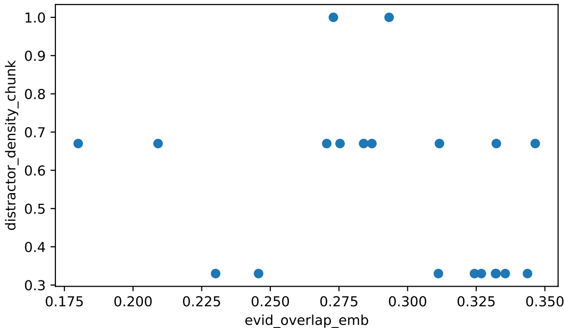
evid_overlap_emb vs distractor_density_chunk Spearman rho=-0.322 (weak), n=20
