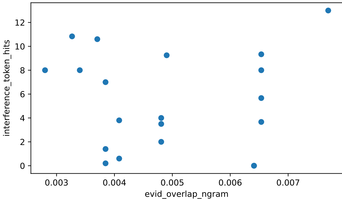
evid_overlap_ngram vs interference_token_hits Spearman rho=-0.044 (weak), n=20
