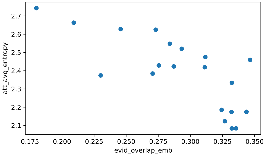
evid_overlap_emb vs att_avg_entropy Spearman rho=-0.690 (moderate), n=20
