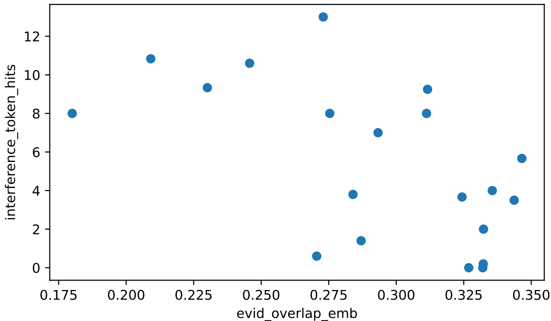
evid_overlap_emb vs interference_token_hits Spearman rho=-0.570 (moderate), n=20
