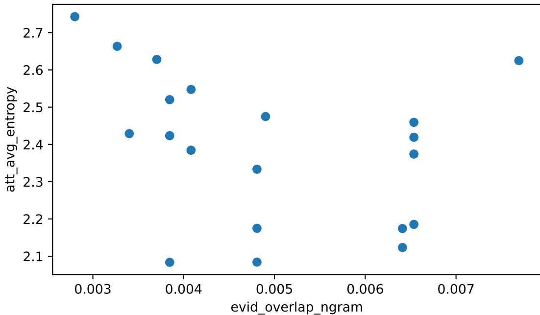
evid_overlap_ngram vs att_avg_entropy Spearman rho=-0.363 (weak), n=20
