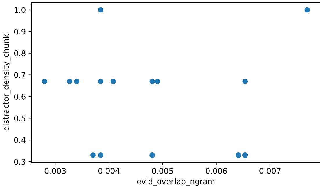
evid_overlap_ngram vs distractor_density_chunk Spearman rho=-0.240 (weak), n=20
