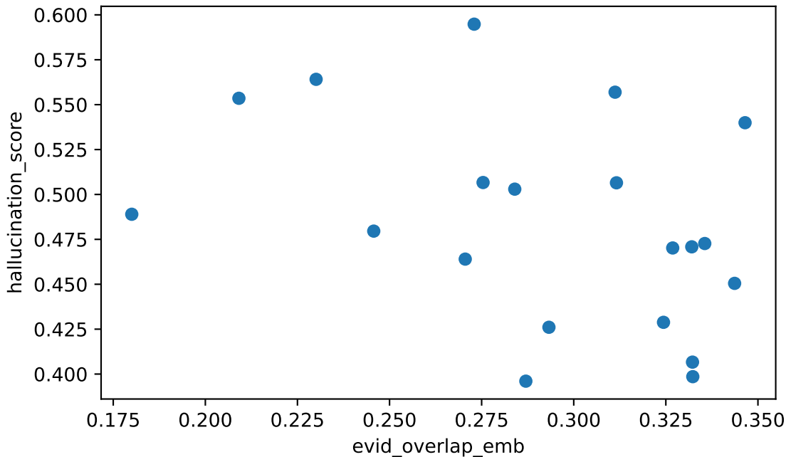
evid_overlap_emb vs hallucination_score Spearman rho=-0.408 (moderate), n=20
