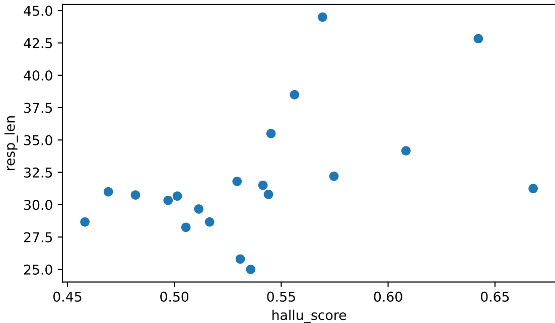
hallu_score vs resp_len Spearman rho=+0.643 (moderate), n=20
