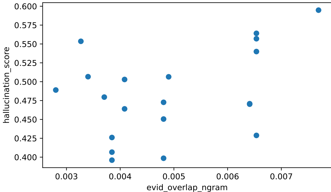
evid_overlap_ngram vs hallucination_score Spearman rho=+0.287 (weak), n=20
