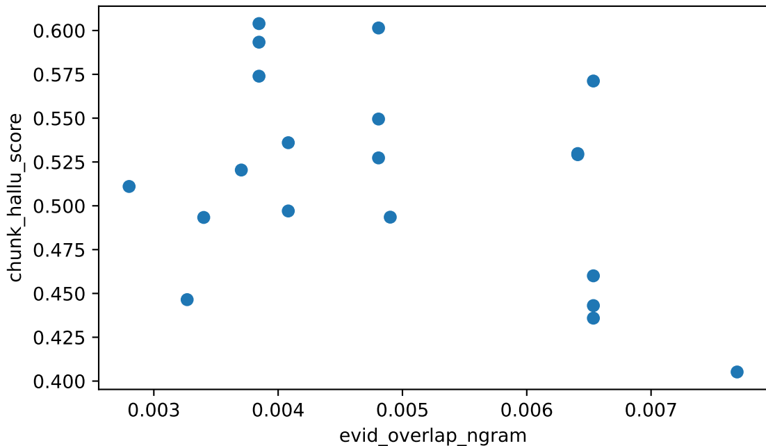
evid_overlap_ngram vs chunk_hallu_score Spearman rho=-0.287 (weak), n=20
