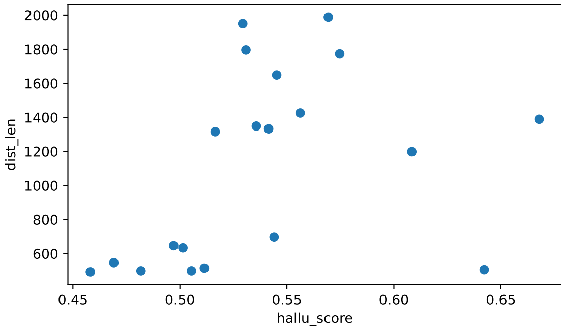
hallu_score vs dist_len Spearman rho=+0.556 (moderate), n=20
