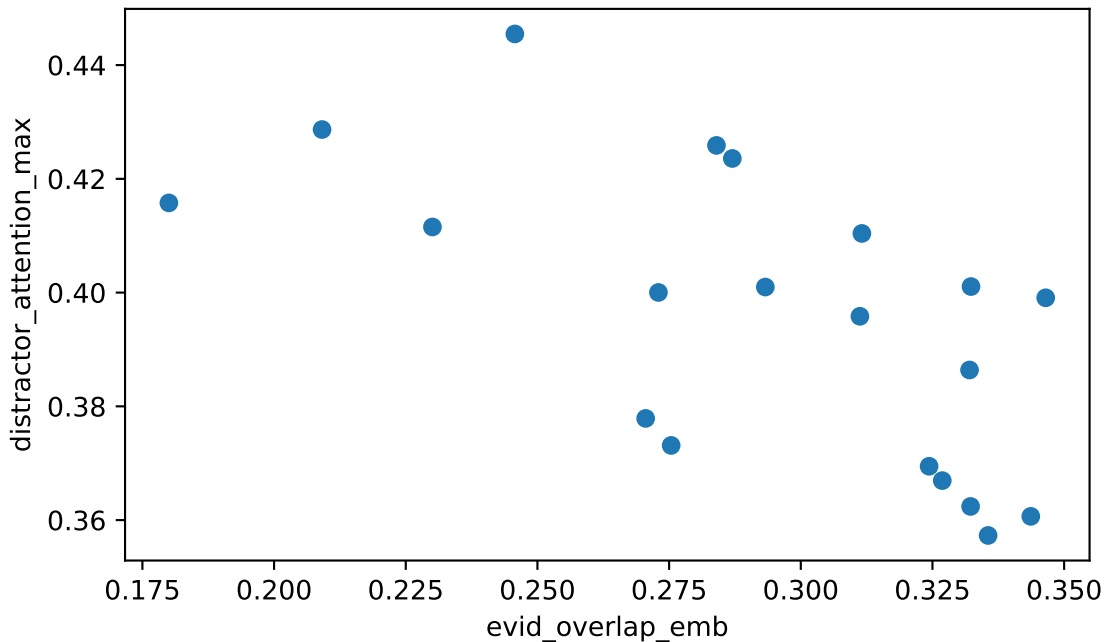
evid_overlap_emb vs distractor_attention_max Spearman rho=-0.651 (moderate), n=20
