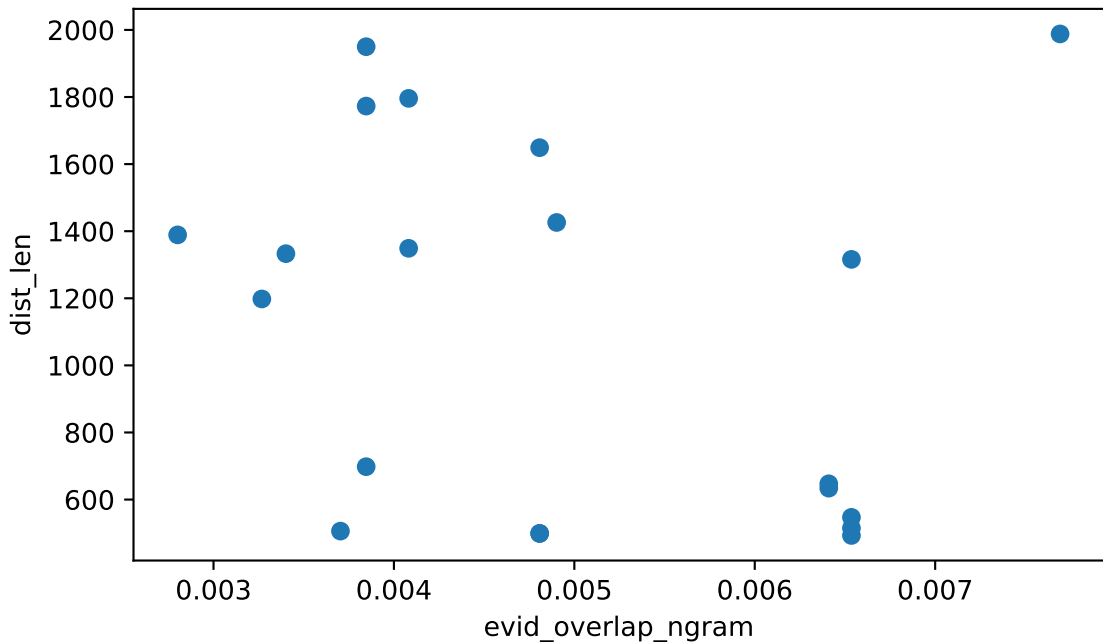
evid_overlap_ngram vs dist_len Spearman rho=-0.211 (weak), n=20
