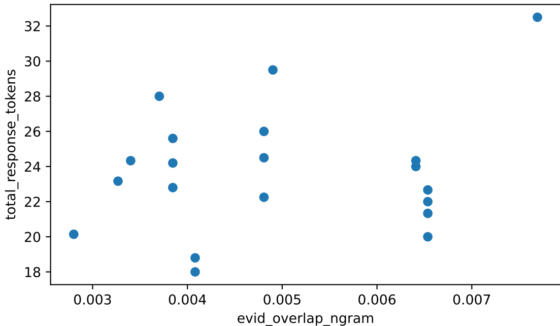
evid_overlap_ngram vs total_response_tokens Spearman rho=-0.007 (weak), n=20
